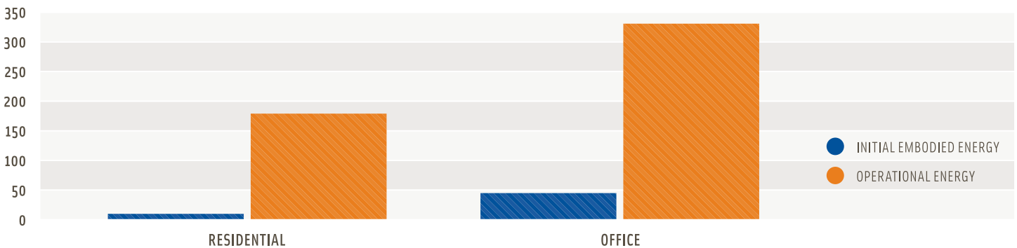
FIG. 7. The operational phase of any building far outweighs the construction phase in terms of energy use over a typical service life, such as 50 years, and the longer the building is in operation, the greater the benefit.
