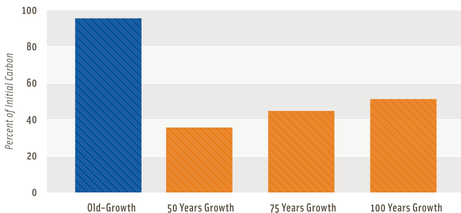
FIG. 11. When trees in a frontier forest are harvested for use, it requires several centuries to recapture carbon.
