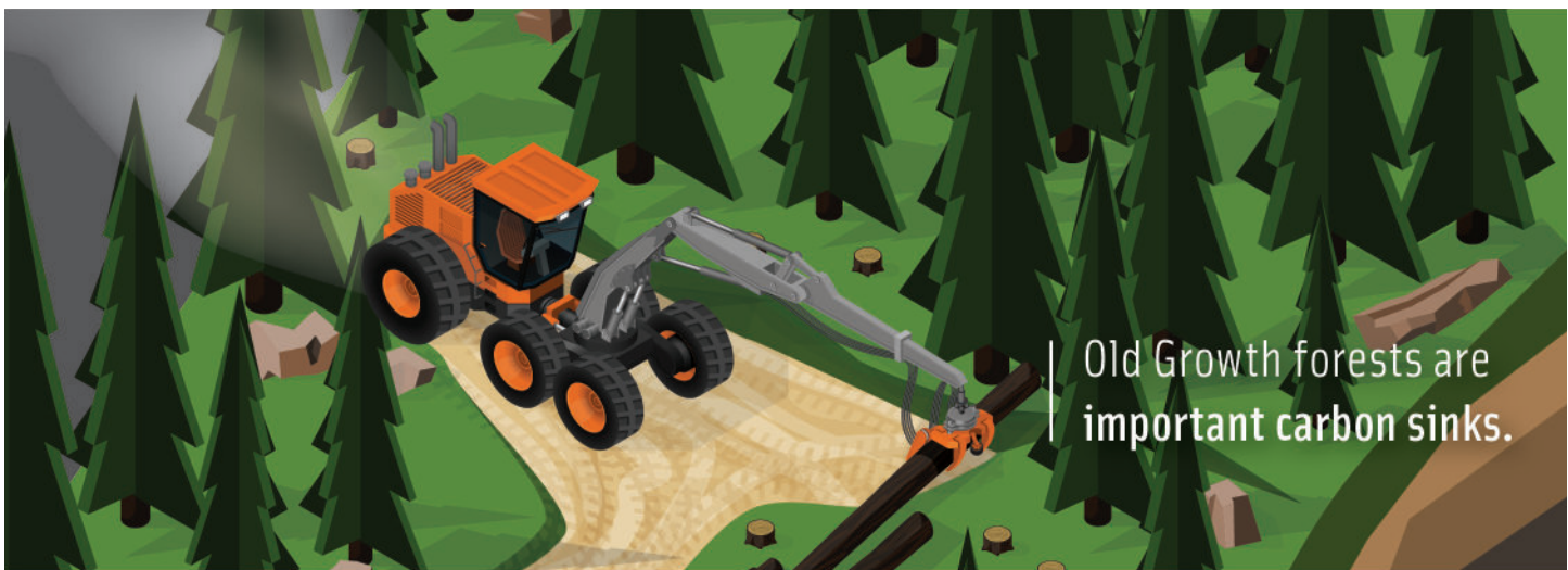
FIG. 10. Frontier forests store substantial amounts of carbon.
