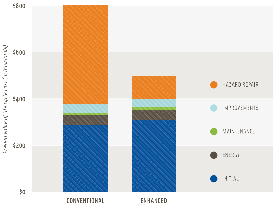
FIG. 6. The chart compares life cycle cost of a conventional and enhanced design for a two-story wood-frame single-family townhouse in the hurricane-prone city of New Orleans. Over a 50-year life, the expected cost of maintaining a conventional building to repair damage from hazards can exceed initial construction costs. By contrast, the enhanced building has slightly higher initial costs but significantly lower hazard repair costs.
